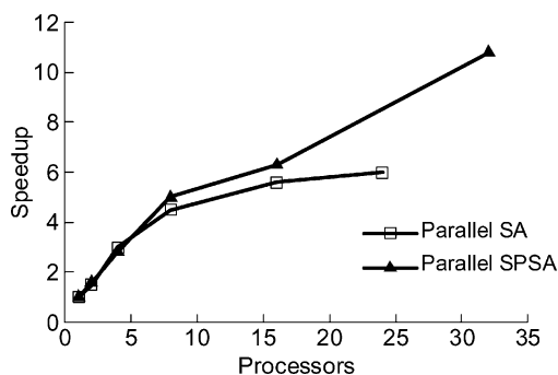
Fig. 4 Comparison of the speedup of parallel SPSA and parallel SA.
