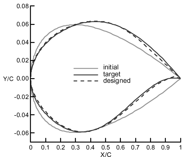
a) Airfoil shapes
