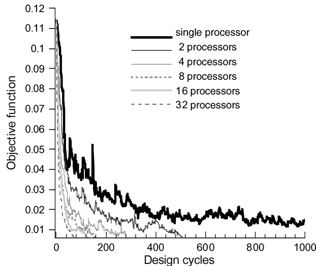
Fig. 3 Convergence histories using parallel SPSA.
