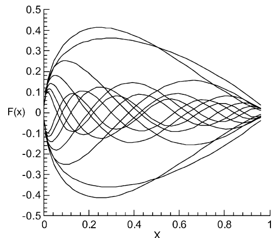
Fig. 1 Plot of Wagner functions.
