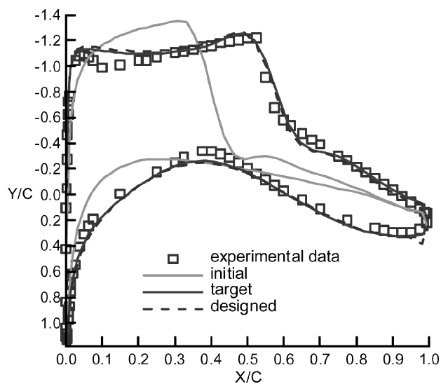
b) Airfoil surface-pressure distributions
