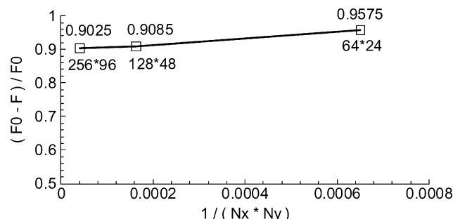
Fig. 2 Influence of grid size on the objective function values.
